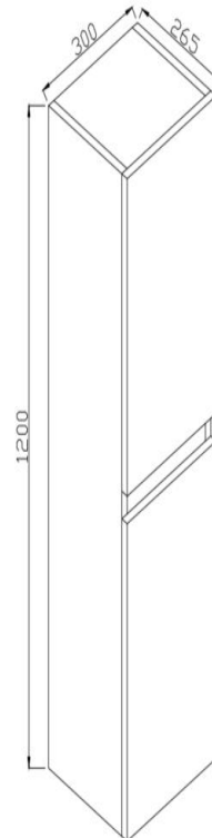
Dimensions (measurements in mm)
